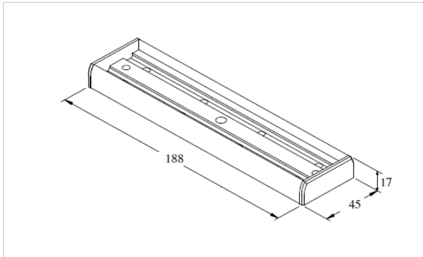
600 LBS EM LOCK AH-275 ARMATURE HOUSING Dimension : 188mm (L) X 45mm(W) X 17mm(H)
